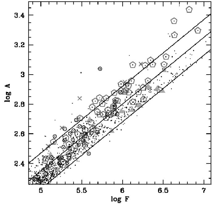
Fig. 2. F - A diagram for the detected sources (dots). Pentagons are confirmed globular clusters, filled triangles are confirmed stars, and small open circles are the previously known candidate globular clusters from the RBC. Crosses are our new candidate clusters.
