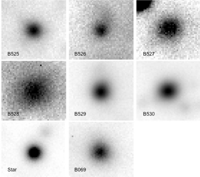
Fig. 3. U images of the six new candidate clusters, a star ( U \sim 18.5 mag) and a confirmed globular cluster with U \sim 18.8 mag (B069). Notice that B069 is one of the blue luminous compact clusters (BLCCs) recently found by Fusi Pecci et al. (2005). Each image is \sim 10'' on a side.
