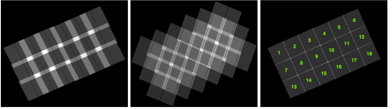
Figure 5. Maps of the relative exposure times across a brick for the WFC3/UVIS (left), ACS/WFC (middle), and WFC3/IR (right) tilings. The labeling of PHAT “fields” within a brick is shown superimposed on the WFC3/IR tiling. The left and right 3 \times 3 half-bricks are taken with orientations 180^\circ apart, as can be seen by the relative position of the dark circle in the WFC3/IR exposure map. The WFC3/UVIS exposures are dithered to cover the chip gap. The WFC chip gap in ACS is not dithered within a single orbit, but is covered by overlapping exposures.
