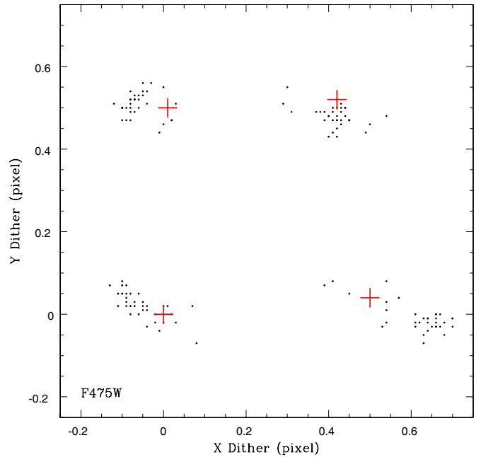
Figure 4. Sub-pixel dithers requested (red crosses) and achieved (points) are shown for ACS/WFC F475W images obtained during the winter 2010 observing season. Note that the requested dithers do not fall exactly at the optimal 2 \times 2 0.5 pixel locations, as the dither sequence operates on both the F475W and F160W filters simultaneously, and thus is a compromise between the needs of the two filters. The deviation of the actual dithers from the ideal interlace pattern is small enough that algorithms that can reconstruct Nyquist-sampled images from non-optimal dithers, such as that of Lauer (1999), should still work satisfactorily.
