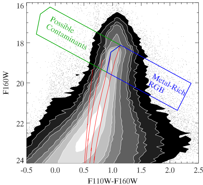
Figure 26. Example of selection of RGB stars from the NIR CMD. The blue selection region selects RGB stars with [\text{Fe}/\text{H}] > -0.7 and reddenings up to E(B - V) = 3 . This metal-rich RGB selection box only includes the brightest stars to ensure uniform selection of RGB stars even in the crowded inner disk (i.e., Figure 11). The green box indicates possible contaminants that could be reddened into the RGB selection area. These contaminants are metal-poor RGB stars, red supergiants, and AGB stars. This box typically contains 25% of the stars in the metal-rich selection box. Red lines indicate RGB positions for [\text{Fe}/\text{H}] = (-2.3, -1.3, -0.7, 0.0) with an age of 10 Gyr. The NIR data are drawn from the merged catalog of Bricks 8 and 9; identical selection criteria were used in all other regions. A foreground extinction correction of E(B - V) = 0.062 was applied to the data before plotting.
