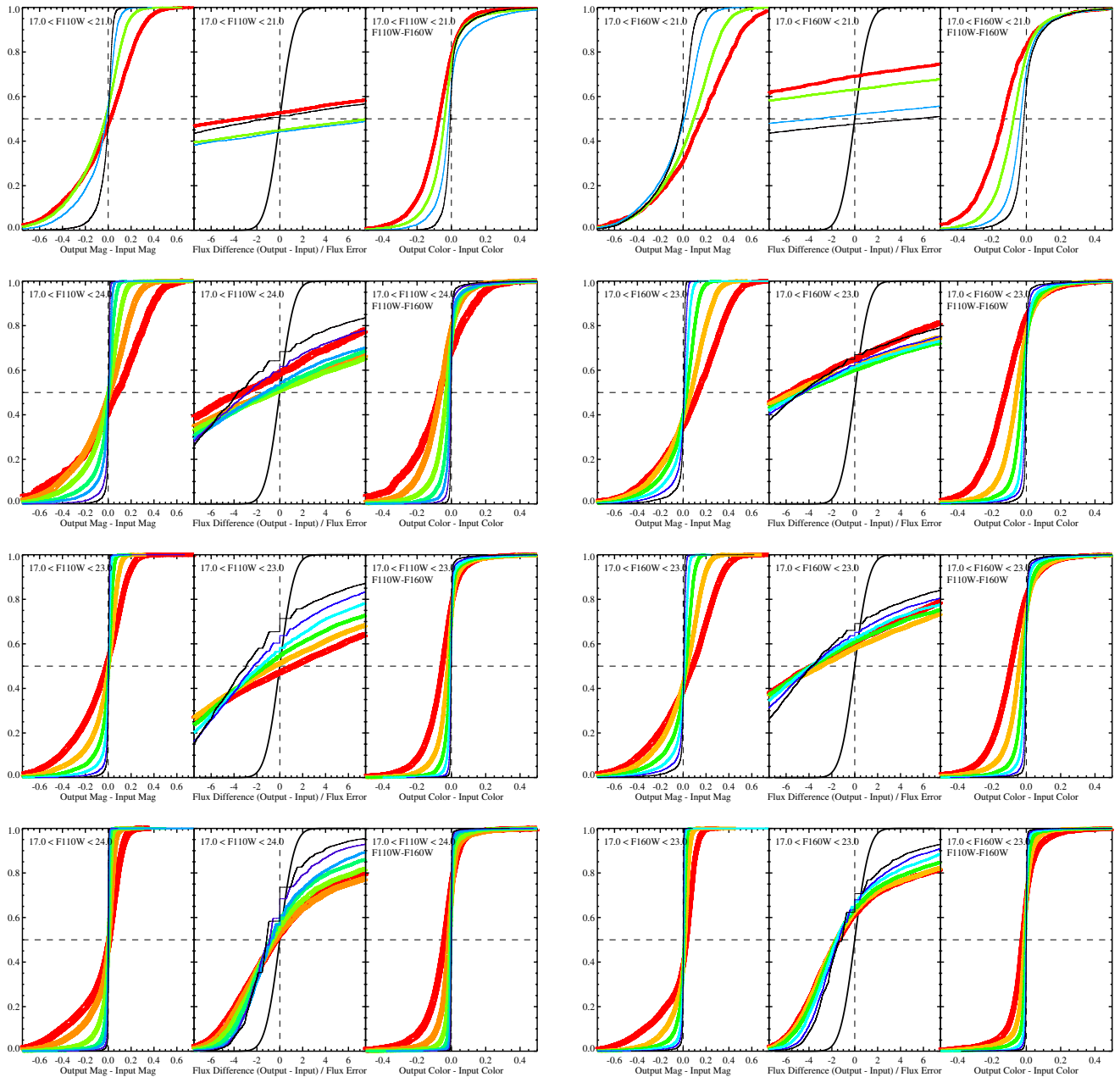
Figure 16. Comparisons between the input and output properties of artificial stars inserted into WFC3/IR images of Brick 1, 9, 15, and 23 (top to bottom respectively), for F110W (left column) and F160W (right column). Panels show the cumulative distribution of (left) the difference between the recovered and inserted magnitude, such that negative numbers indicate stars that are recovered brighter than their true magnitude; (center) the fractional difference in flux, scaled by the photometric uncertainty reported by DOLPHOT such that positive numbers indicate stars that are recovered brighter than their true magnitude; and (right) the difference between the recovered and the input color of the artificial stars, such that positive values indicate stars that are recovered redder than their true color. Line types indicate different bins in recovered magnitude, as described in Figure 14. The WFC3/IR data depart dramatically from a Gaussian due to the effects of crowding, everywhere in the disk (see the middle panel of each three-panel plot). The effect is much worse than in the ACS data, due to the larger WFC3/IR pixel size. Moreover, the median star is recovered with a flux that is significantly fainter than its true flux, although crowding does induce the expected tail to brighter fluxes.
